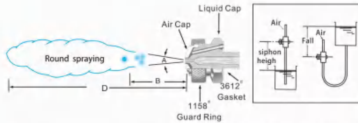
The air cap of round or flat fan pattern produces round or flat fan pattern spraying.
